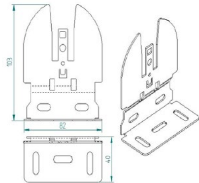
Steel hanger with PCV mask
