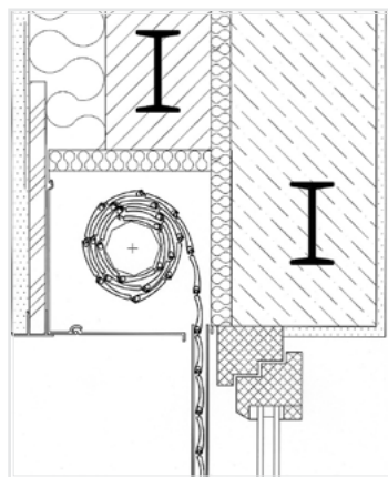
Shutter box built-in the lintel.
