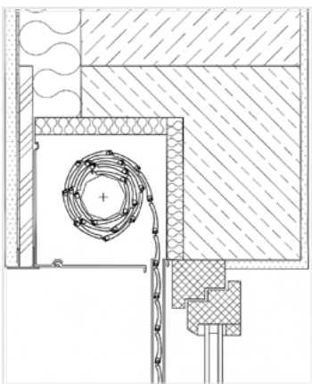
Shutter box built-in the wall.
