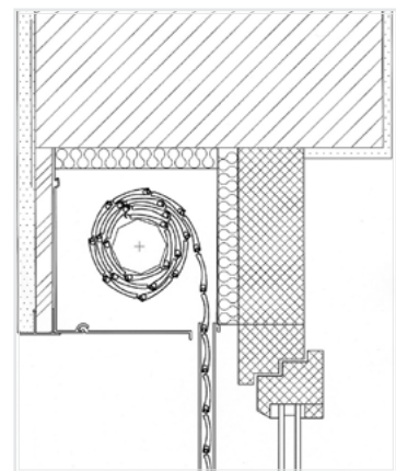
Shutter box built-in under the lintel.
