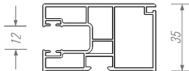
PG 01 - mosquito's guiding rail
