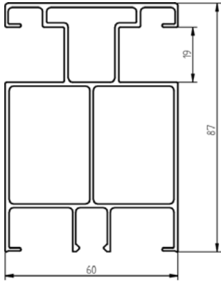
Guide rail PG-10
