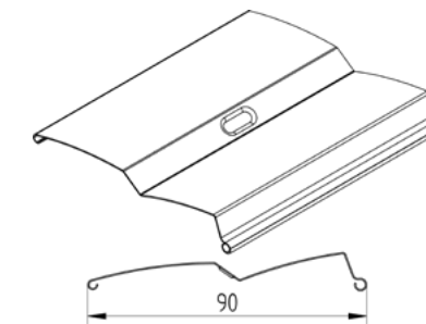
Cross-section of Z-90 lamellas
