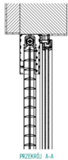
Mounting on the lintel
