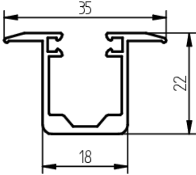
Guide rail PG-12
