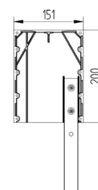
VBox ECO double-sided carrier
