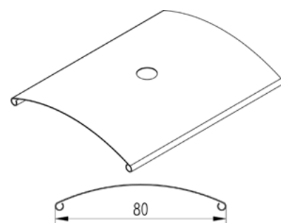
Cross-section of C-80 lamellas
