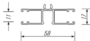
PG 02 - pvc
