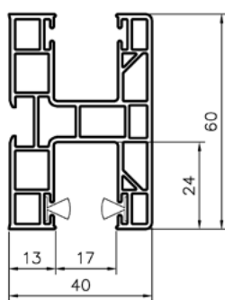
PPDM 60/12
