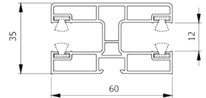
SRM 60 - pvc
