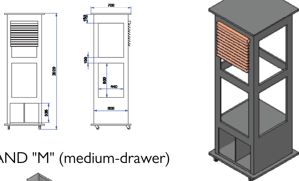
DISPLAY STAND "XL" (extra-large-standing)
