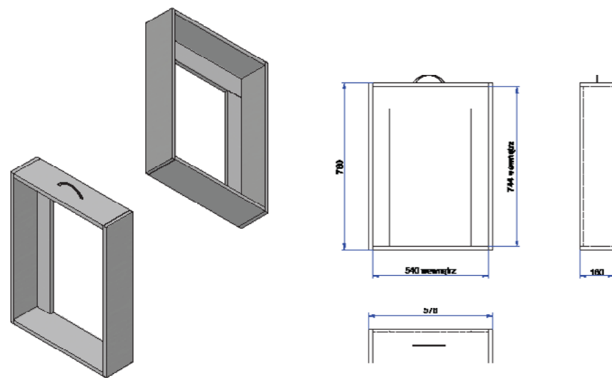
DISPLAY STAND "M" (medium-drawer)
