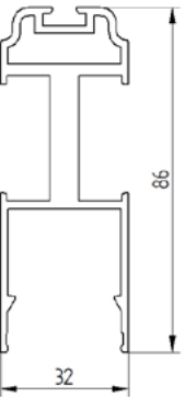
Moving priofile
