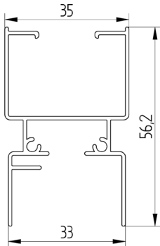
Plisse 20 mm main profile A21
