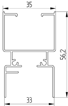
Plisse 20 mm main profile A231
