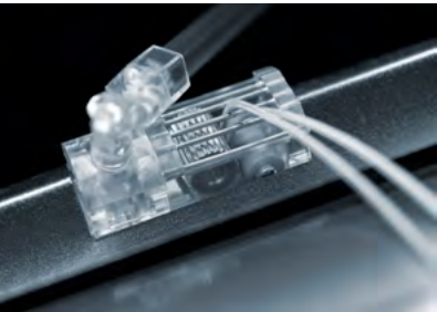
Patent Mechanism
