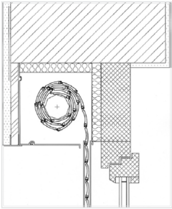
Shutter box built-in under the lintel.
