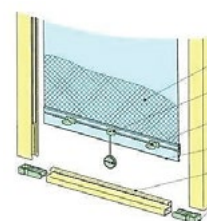
Hakenblockade
